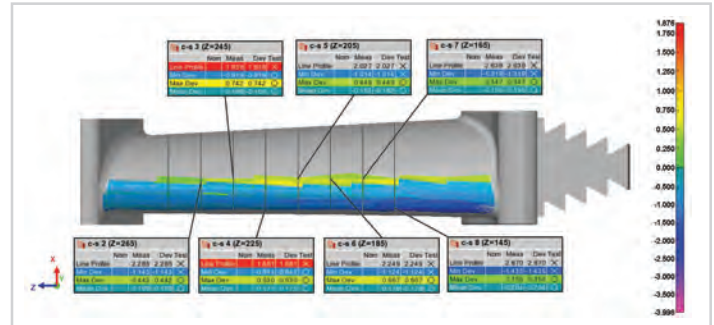
Measurement Profile of Turbine Blade
